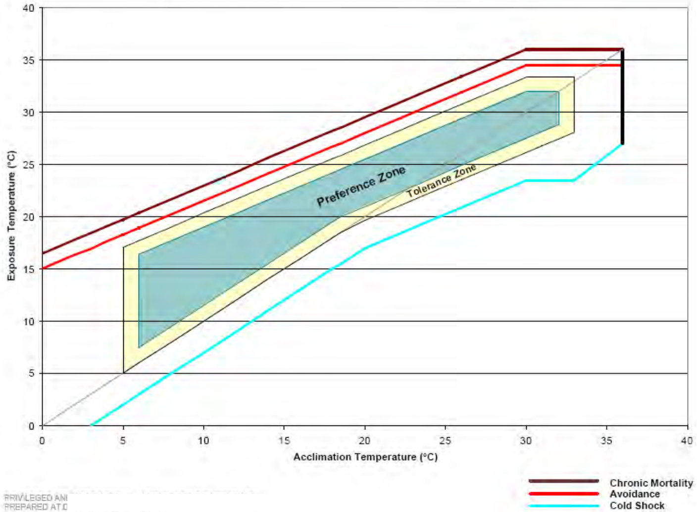
Figure 7. Temperature Tolerance Polygon for Spotfin Shiner
